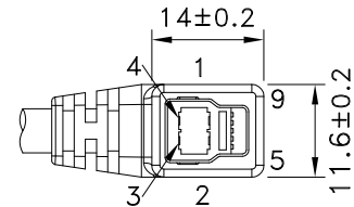
USB B MALE RIGHT ANGLE UP MOLDED BLACK
